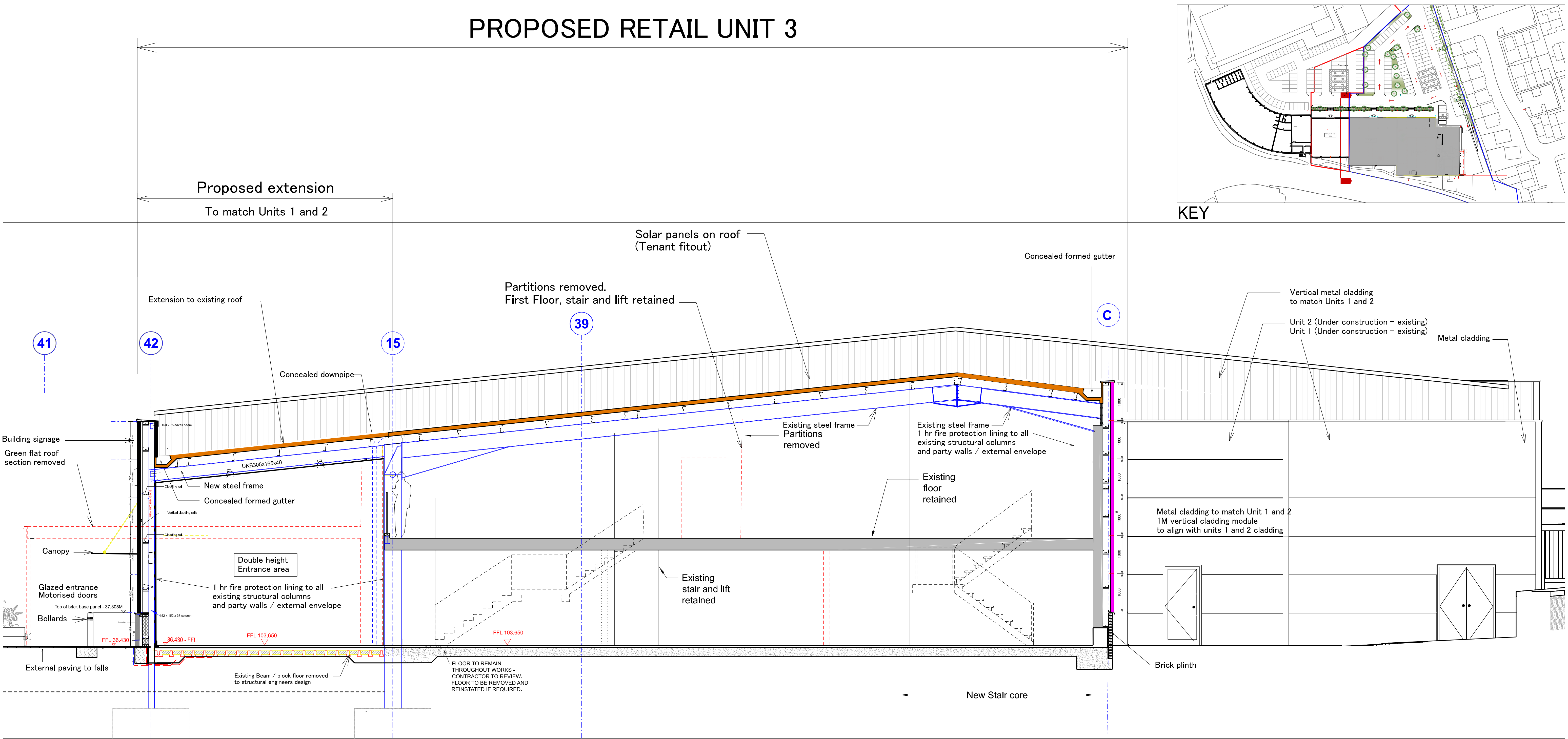
UNIT 3 – PROPOSED SECTION A-A – Through Cladding
