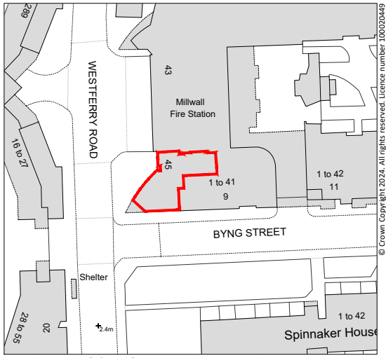
LOCATION PLAN SCALE 1:1250 (GROUND FLOOR)
