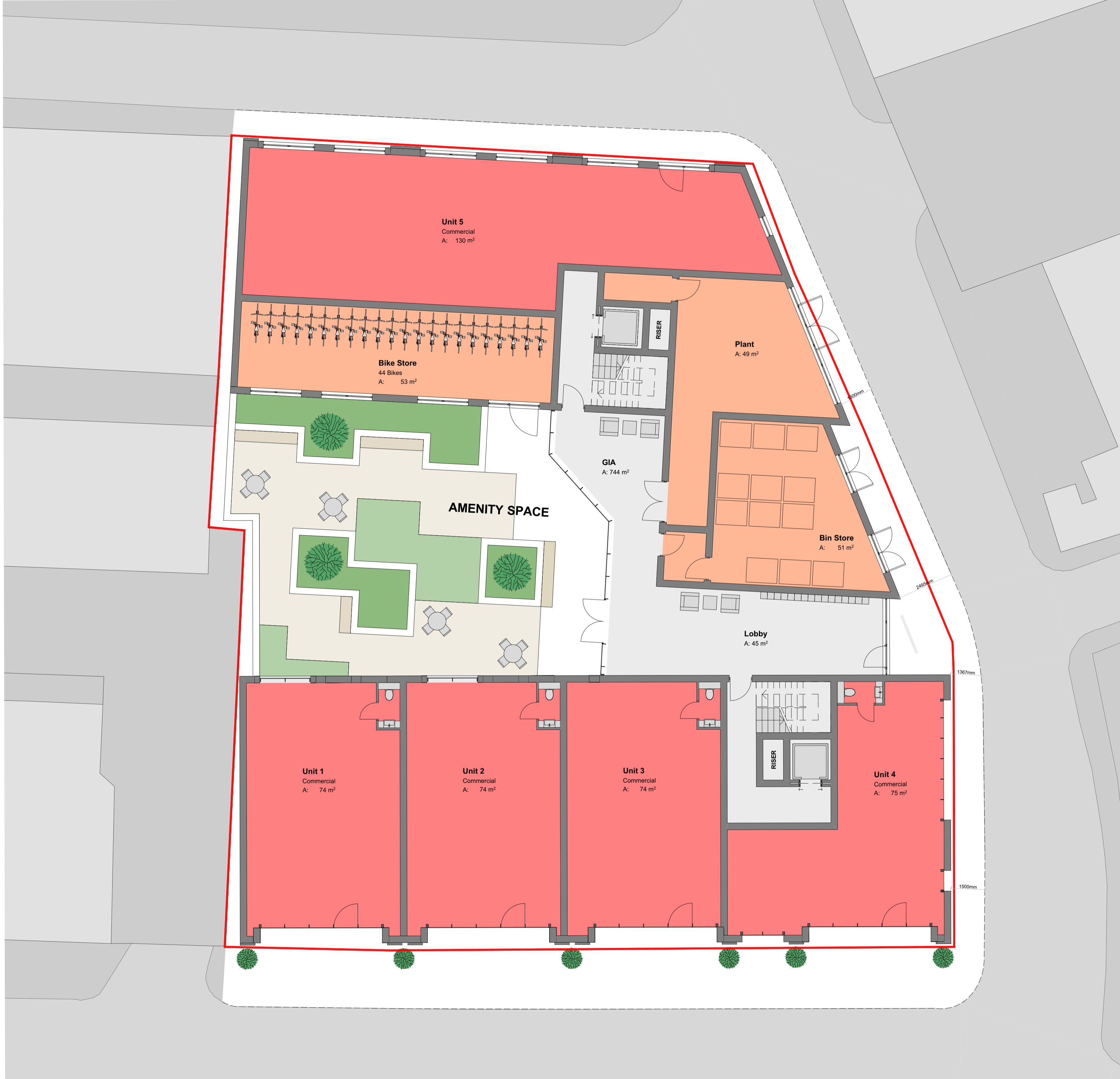
GROUND FLOOR 1:100 @A1
