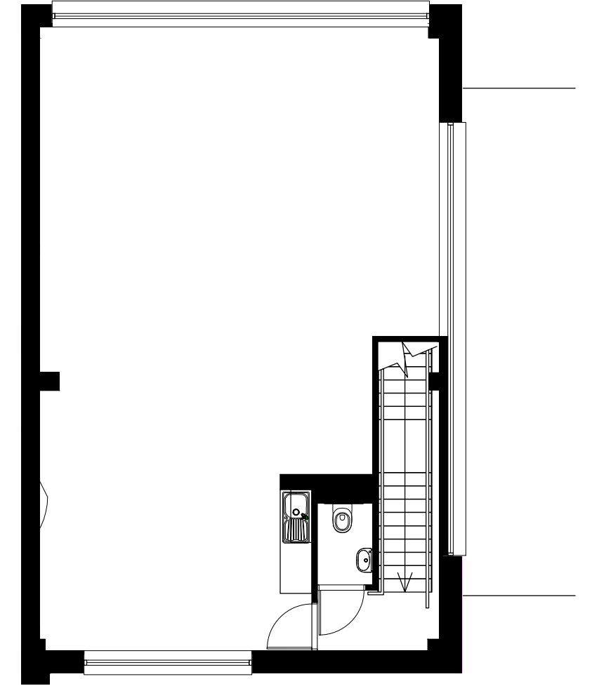
FIRST FLOOR PLAN (1:100 @ A3) 1 0 1 2 3
