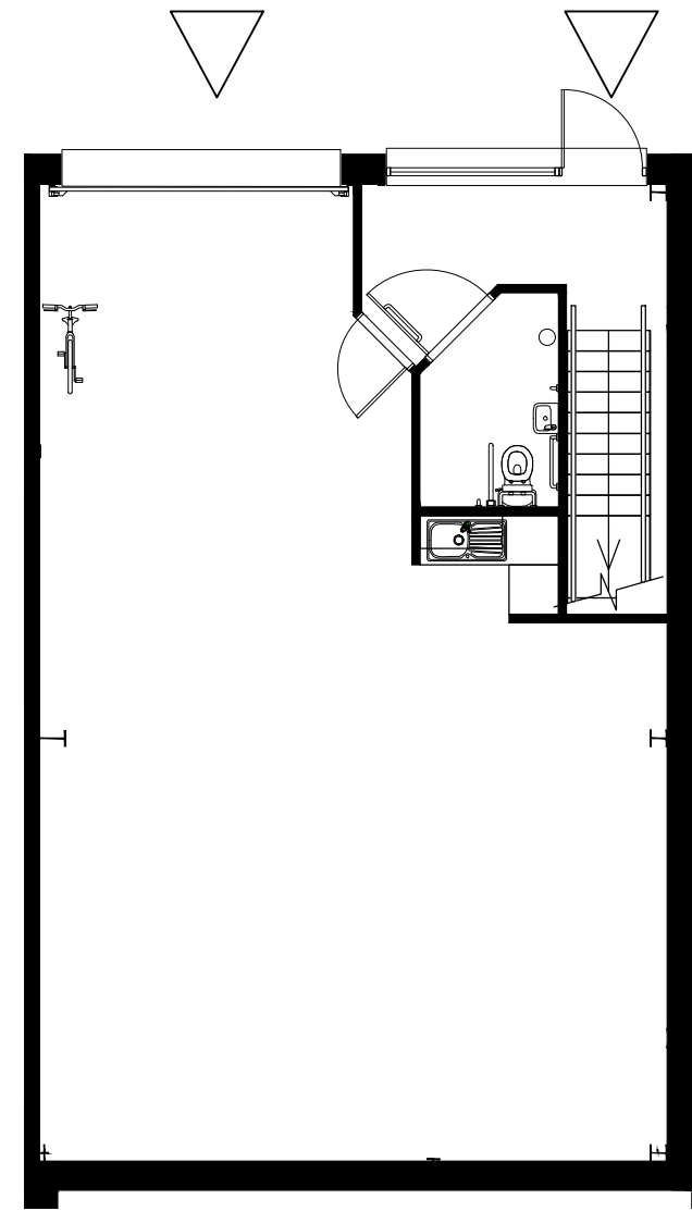
GROUND FLOOR PLAN (1:100 @ A3) 1 0 1 2 3
