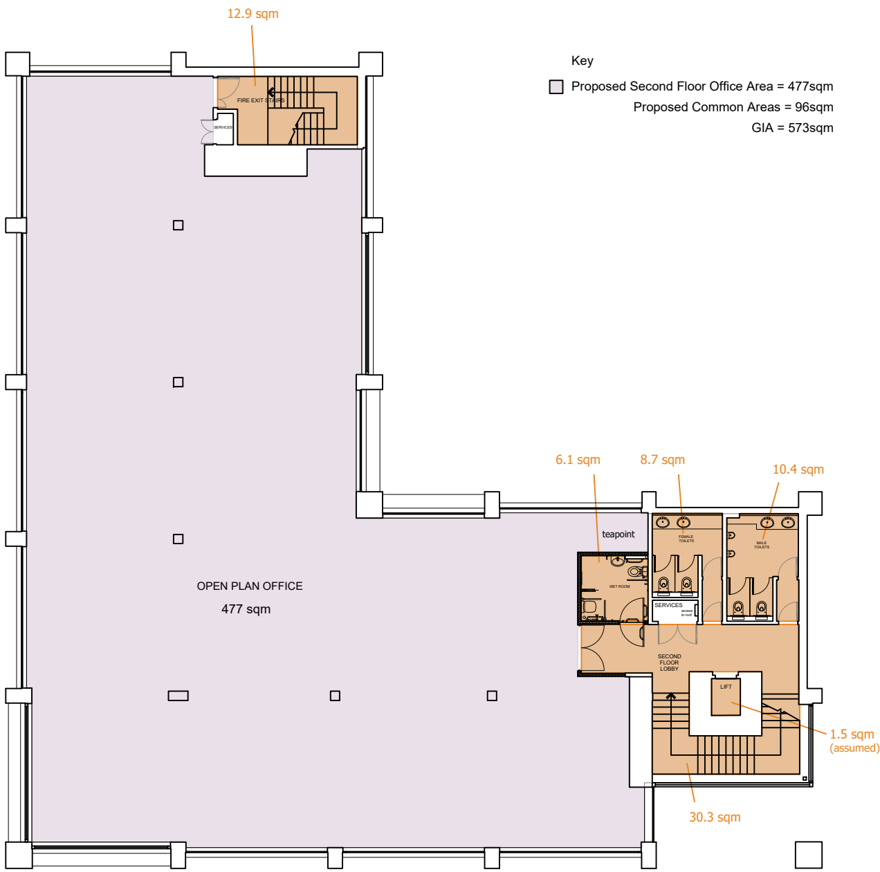
Second Floor
