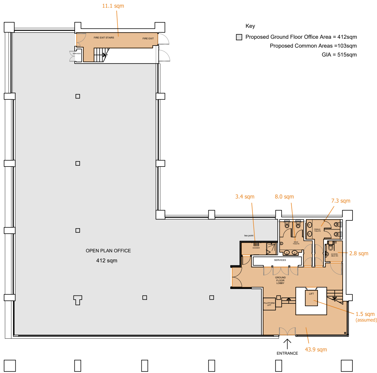
Ground Floor
