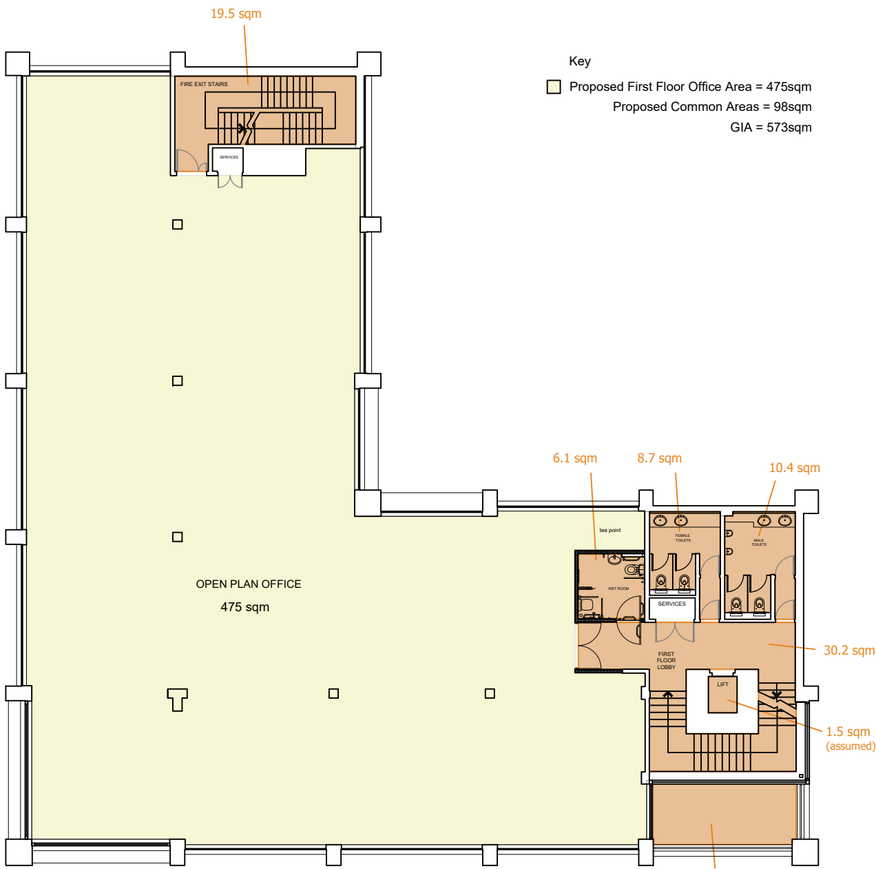
First Floor
