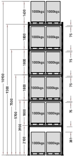
TYPICAL BAY ELEVATION
