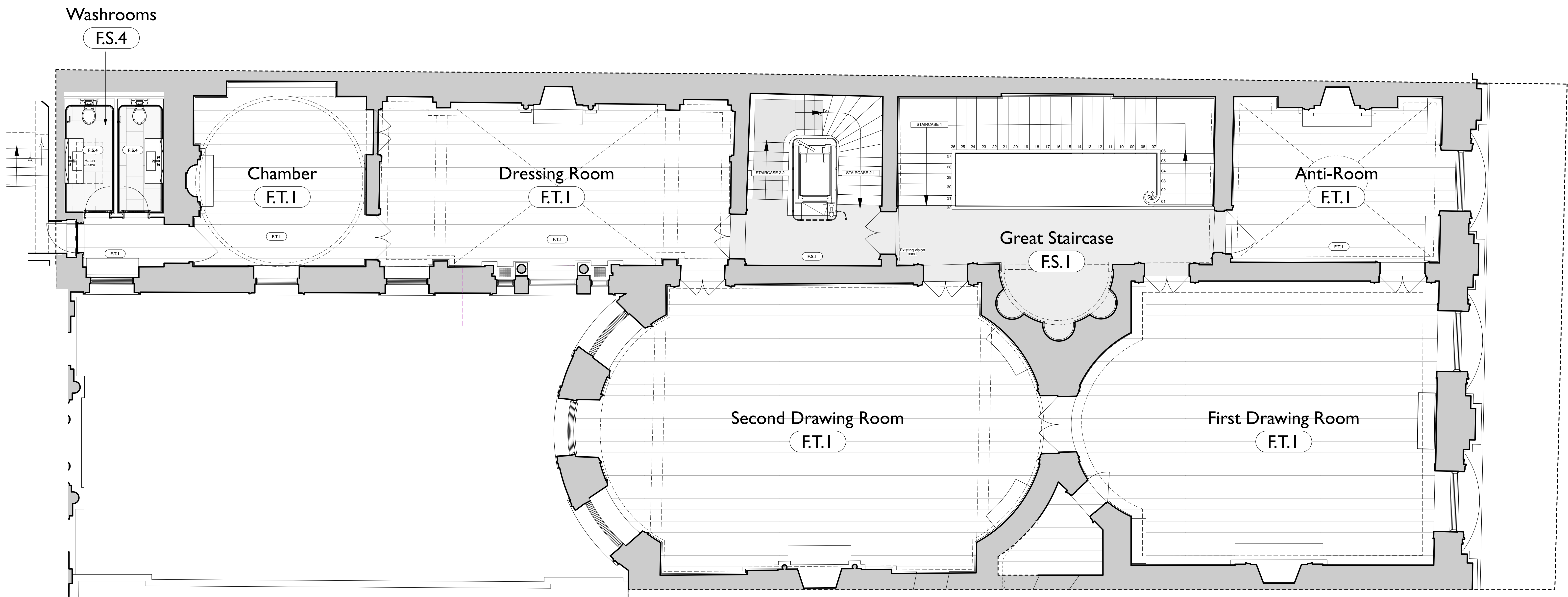
Proposed Plan - First Floor 1:50@A0
