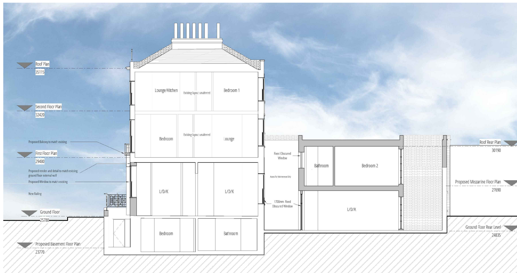
1 Proposed Section BB' 1 : 100
