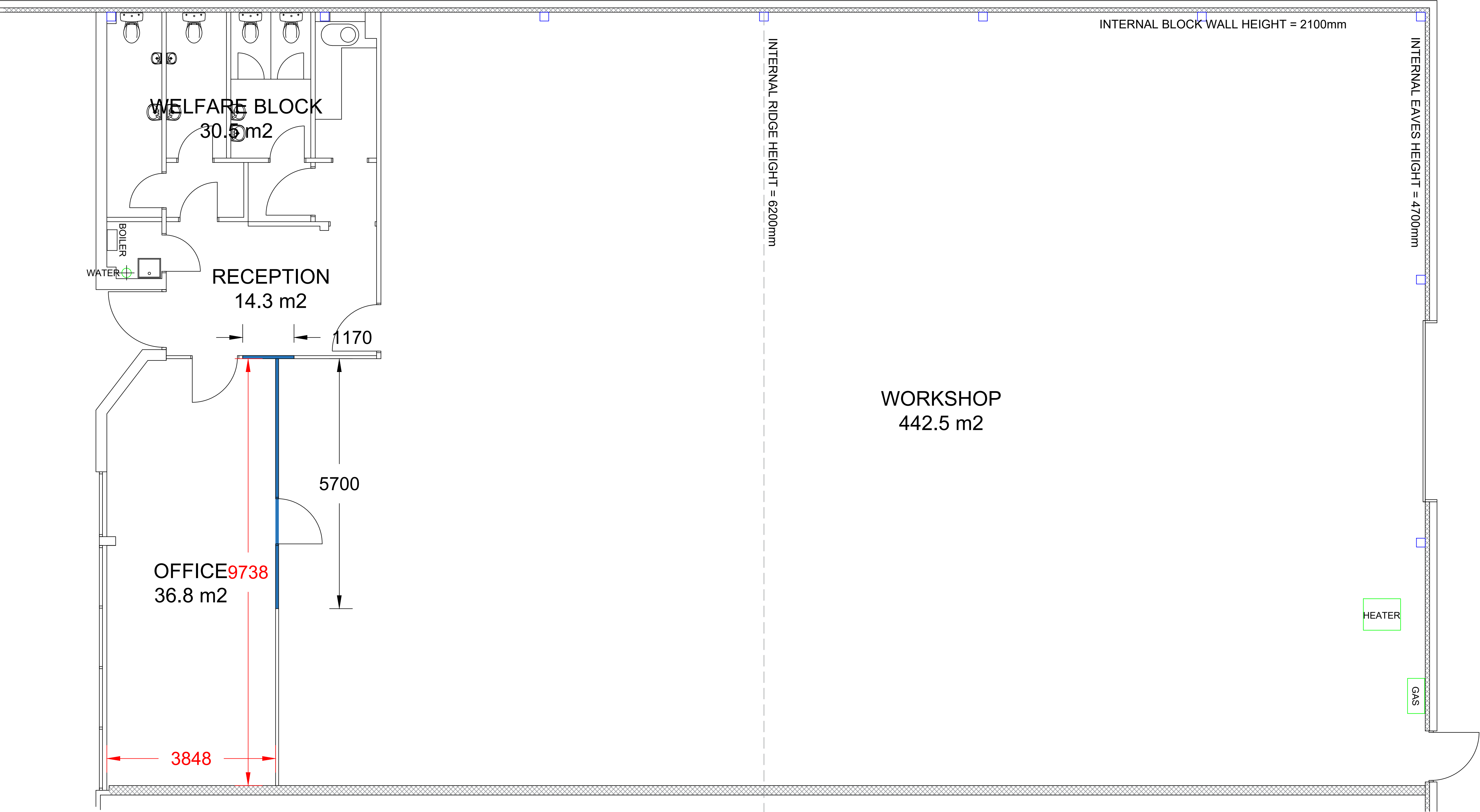
PROPOSED PLAN
