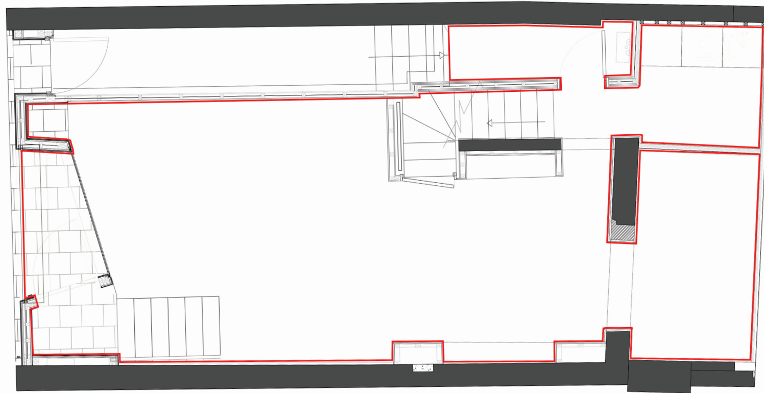
Ground Floor
