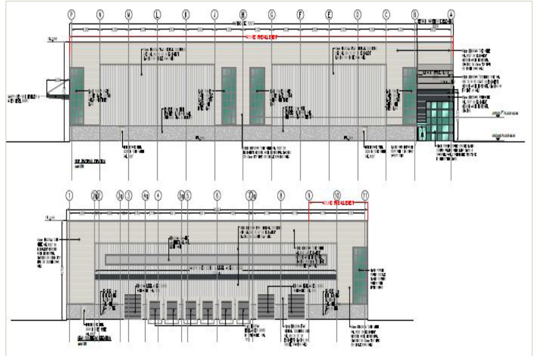
Elevations
