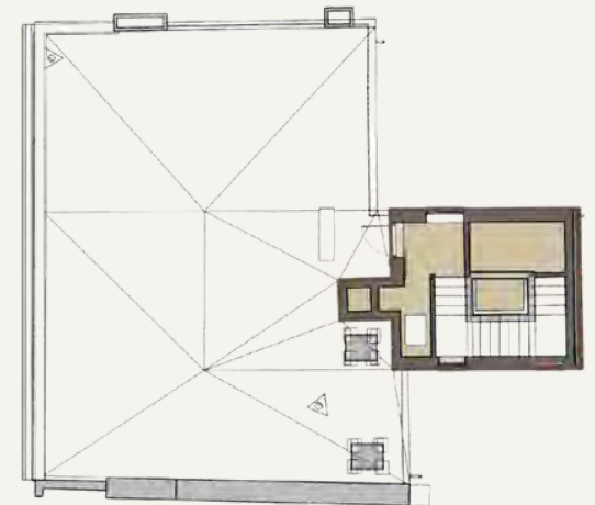
FOURTH FLOOR
