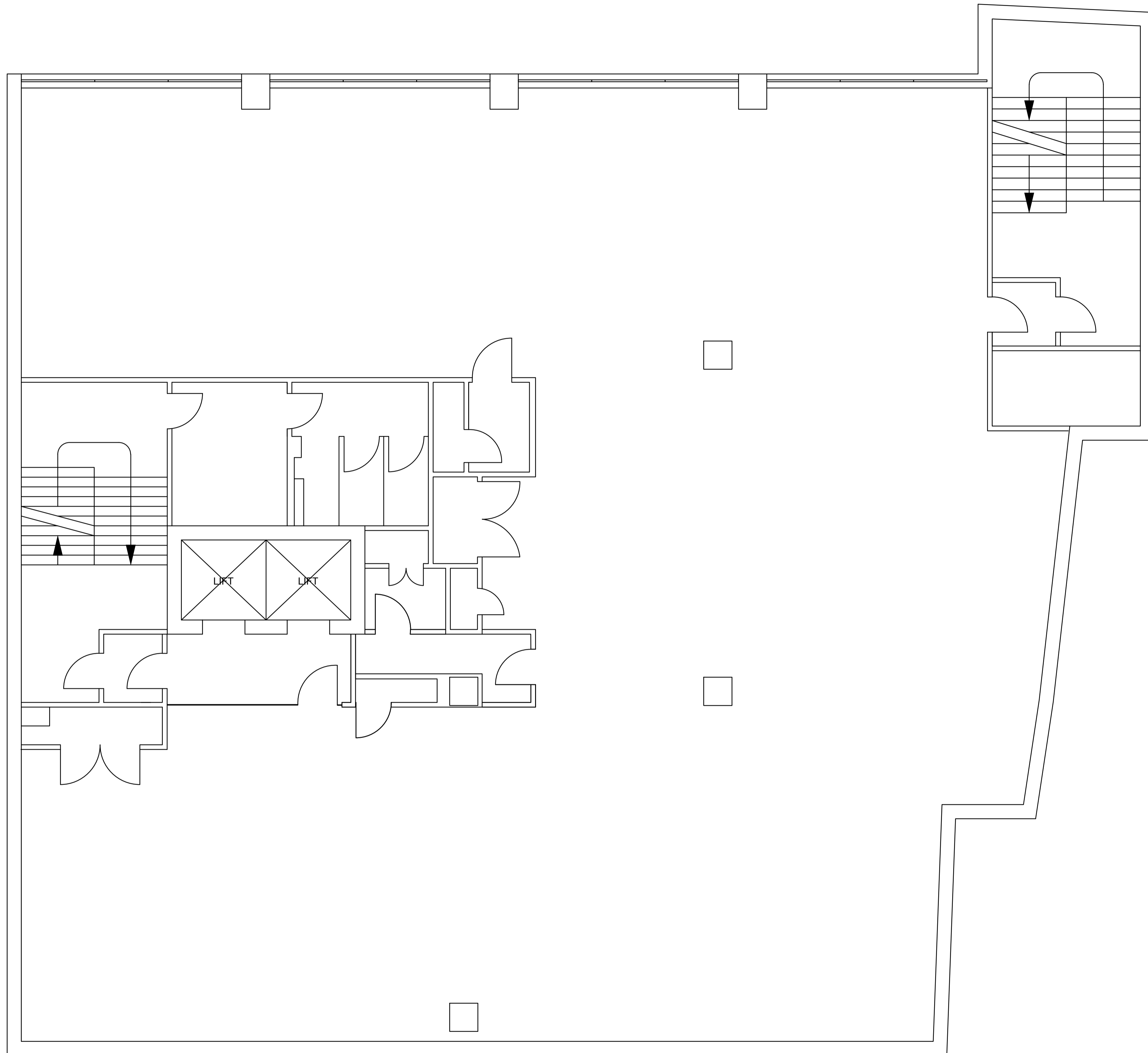
SECOND FLOOR GENERAL ARRANGEMENT SCALE 1:50
