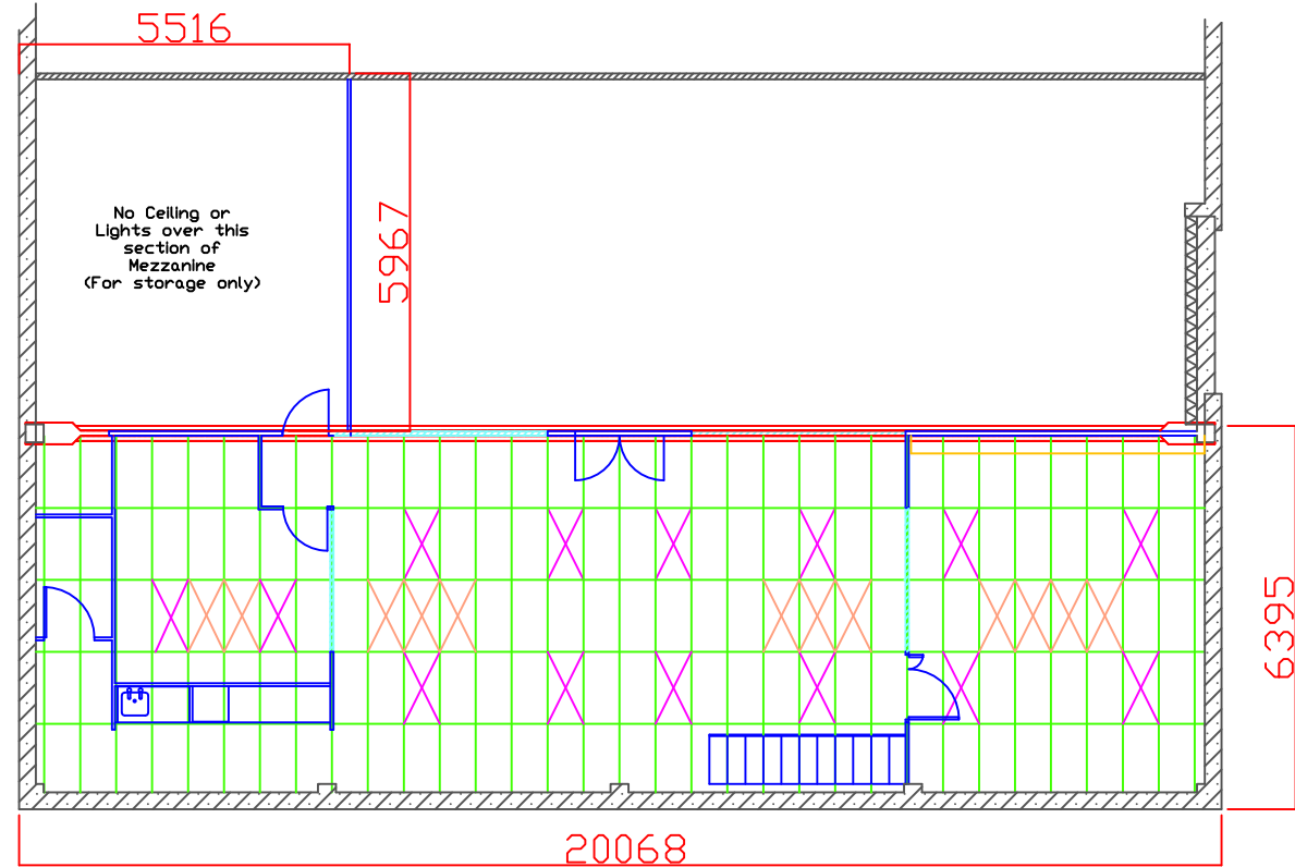
Mezzanine Floor inc. Storage Option
