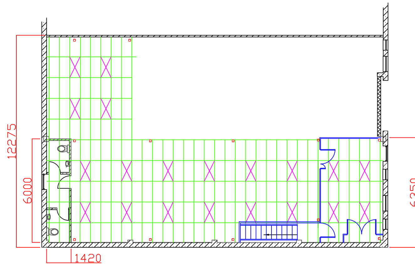
Lower floor - Reflective ceiling plan
