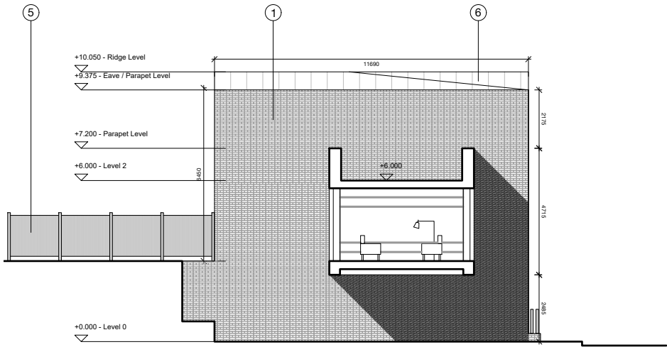
EAST ELEVATION
