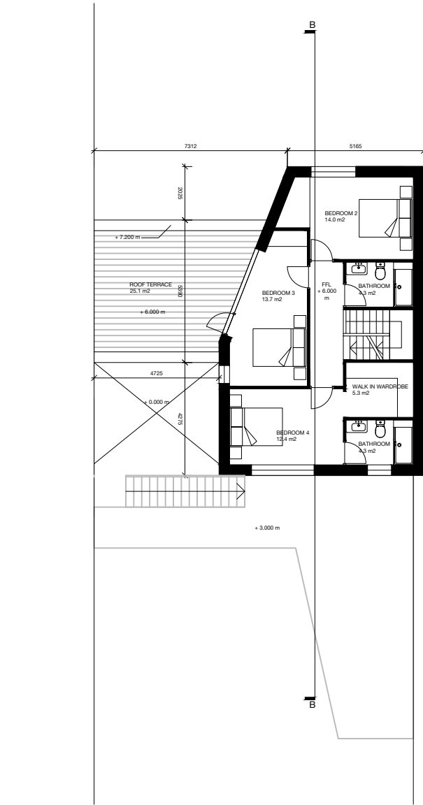
LEVEL 02 PLAN
