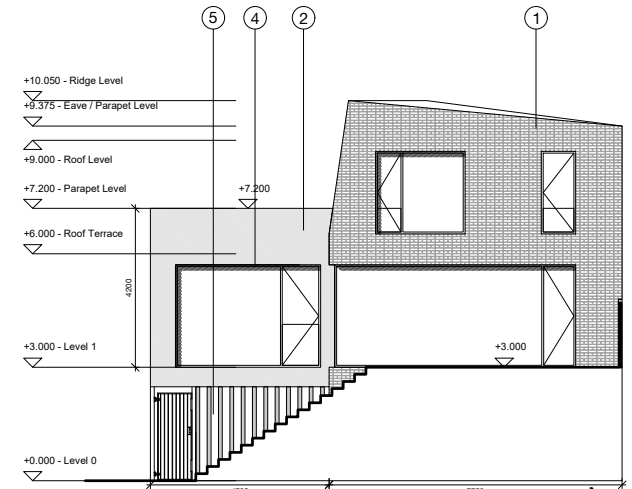
SOUTH ELEVATION
