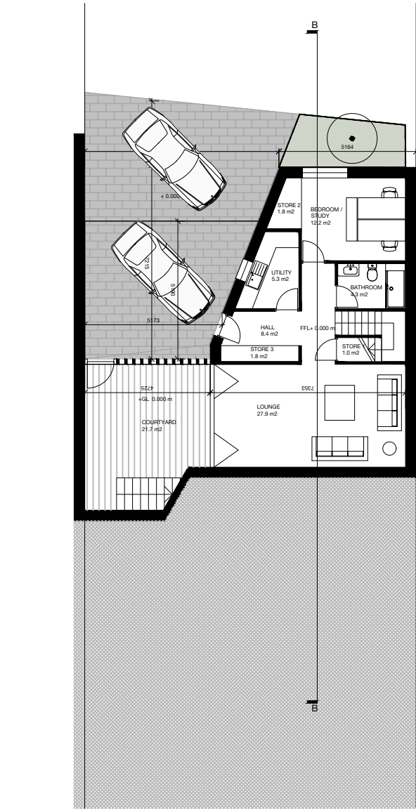
LEVEL 00 PLAN
