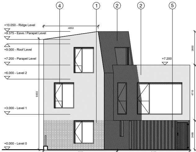
NORTH ELEVATION
