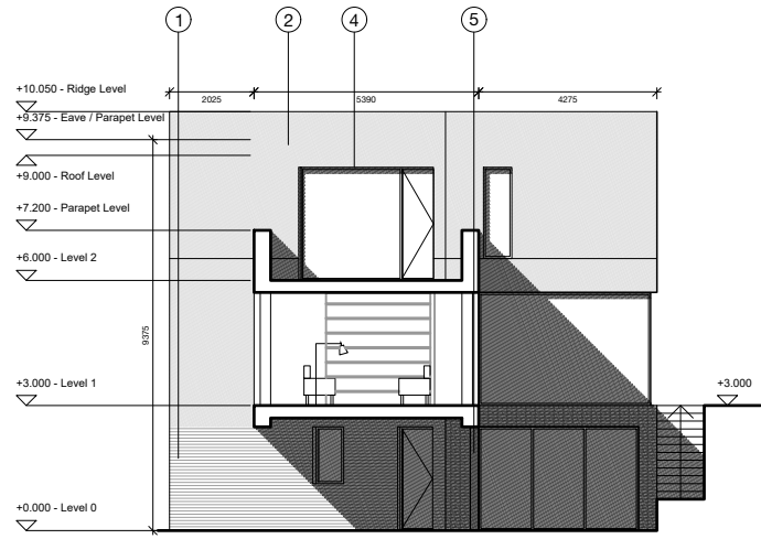
WEST ELEVATION
