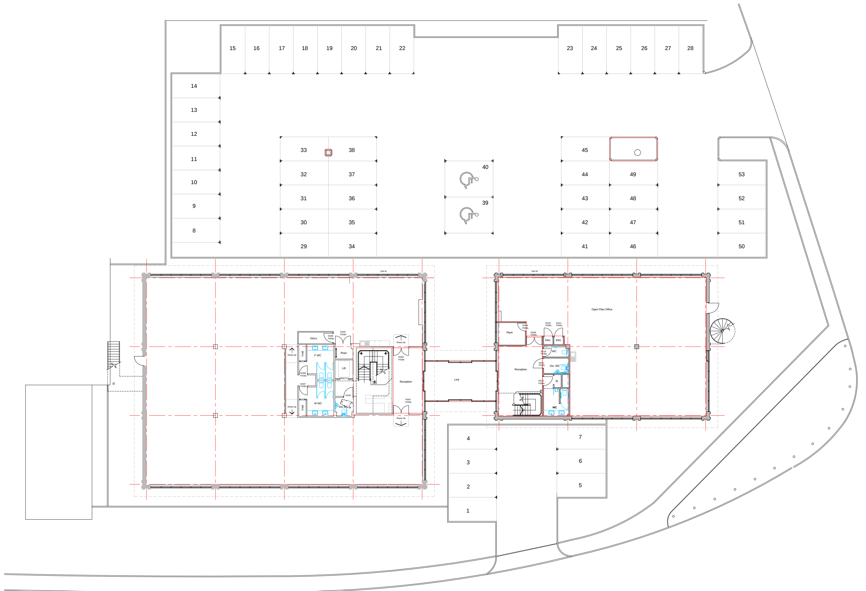
Site Plan and Car Park Layout
