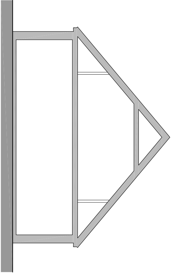
Typical section (proposed) - scale 1/100 0 2m 4m
