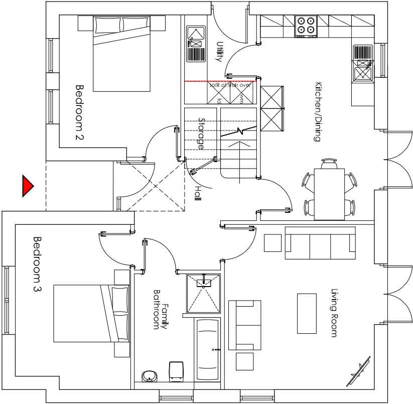
GROUND FLOOR PLAN (proposed) - scale 1/100 0 2m 4m
