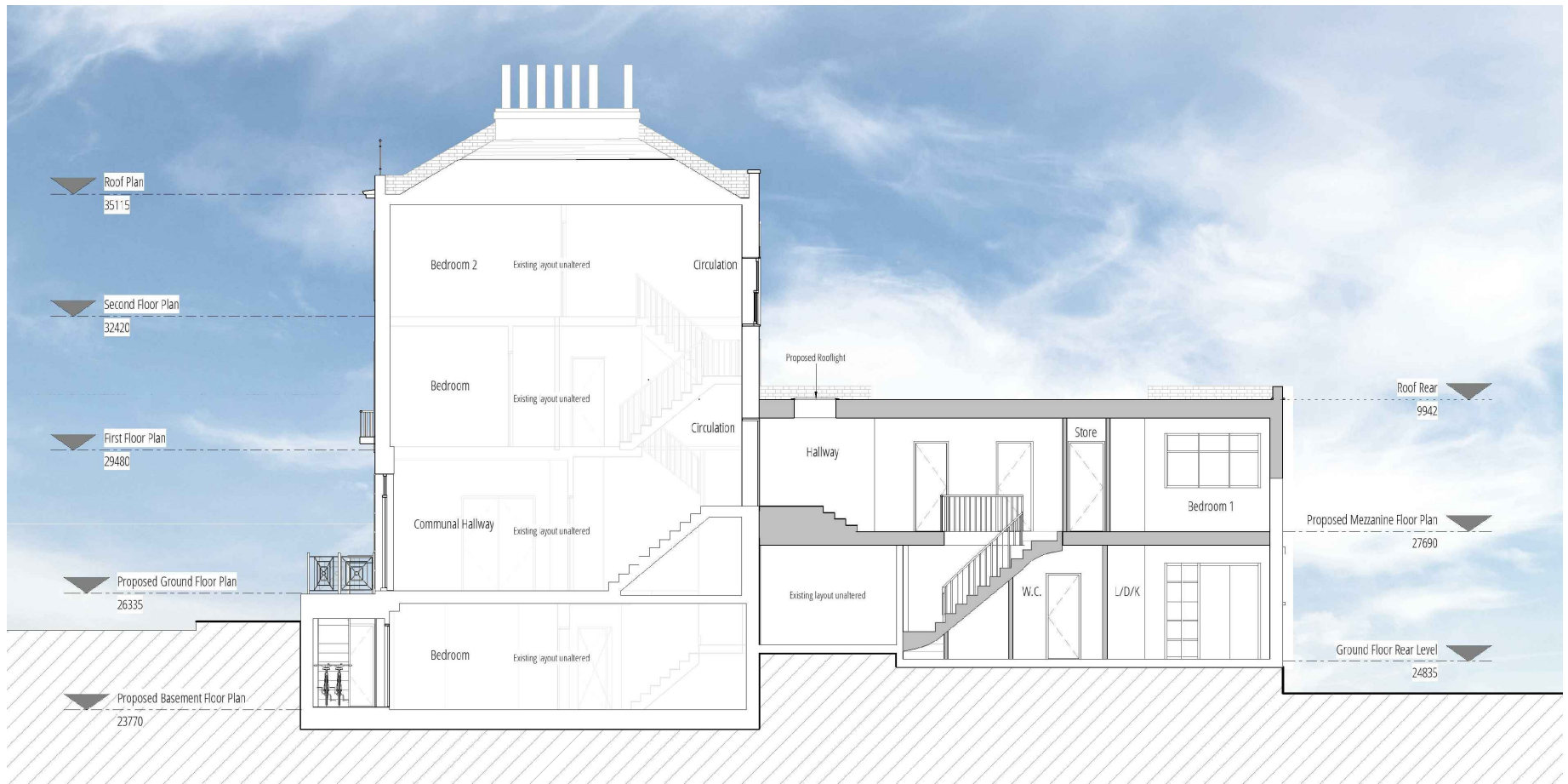
1 Proposed Section CC 1 : 100
