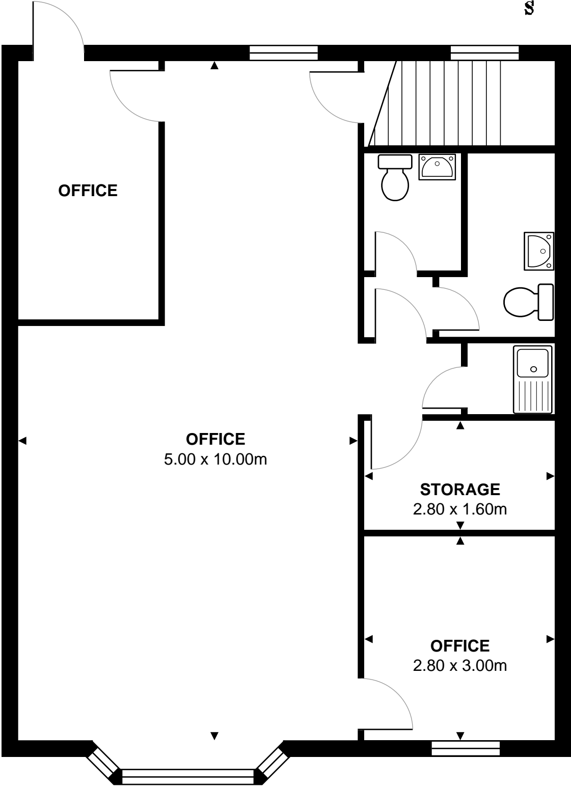
FIRST FLOOR
