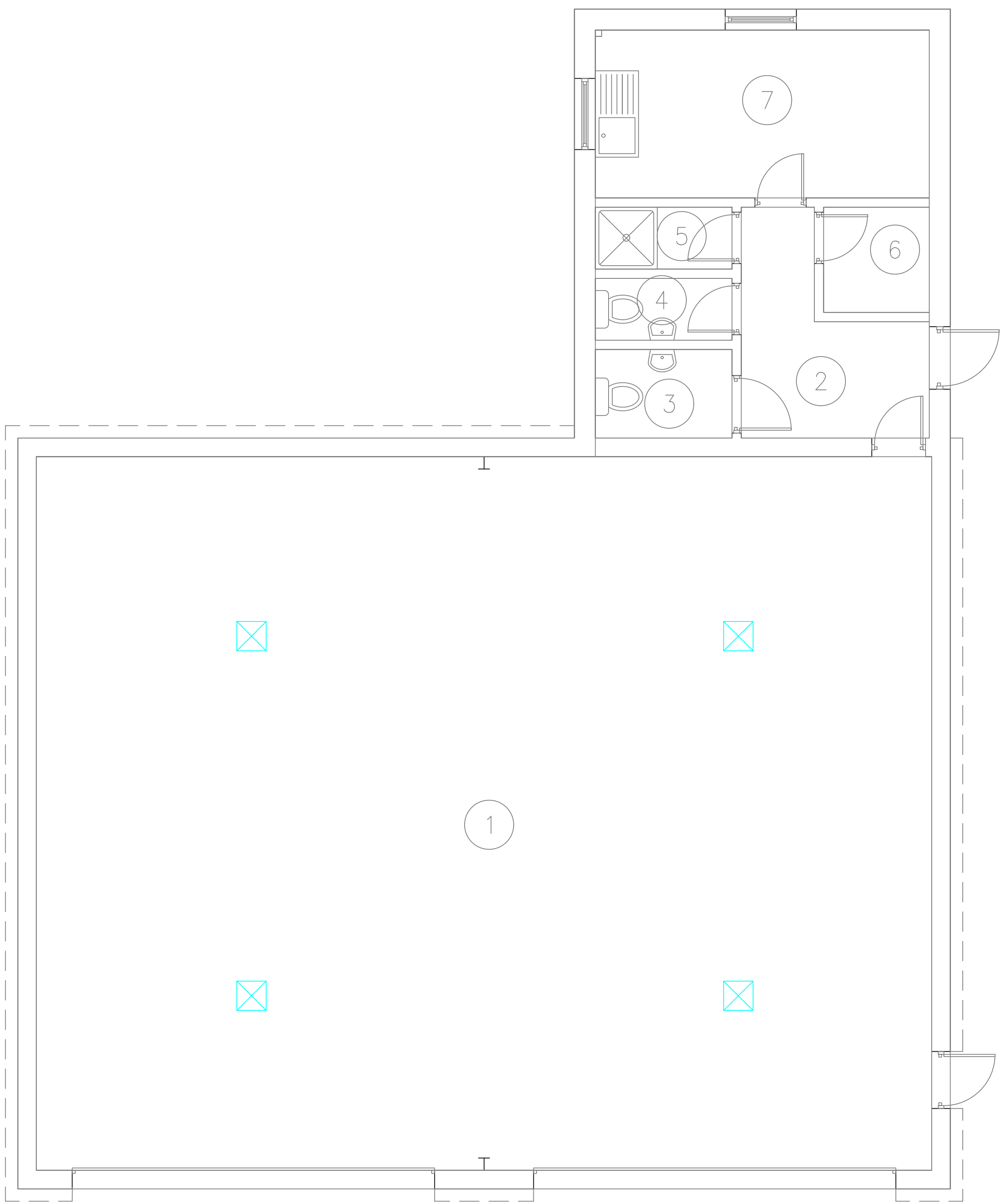
MAIN BUILDING – 0001 GROUND FLOOR
