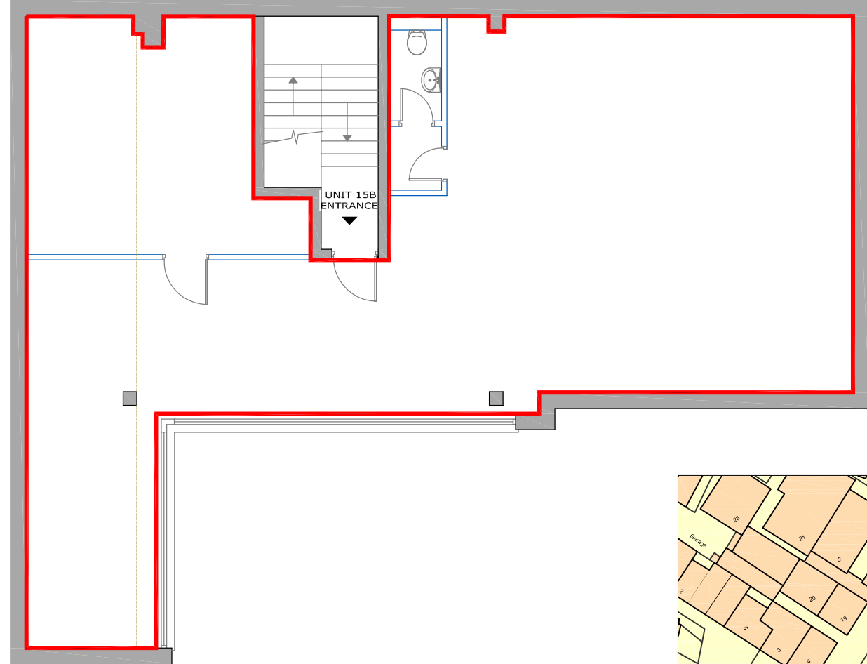
SECOND FLOOR
