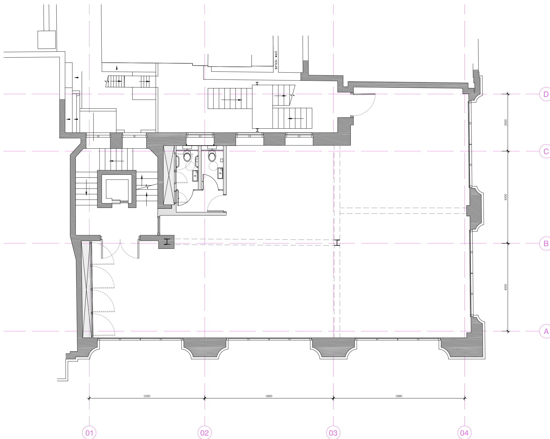
01 Proposed First Floor Plan 20.203 Scale 1:100 @ A3
