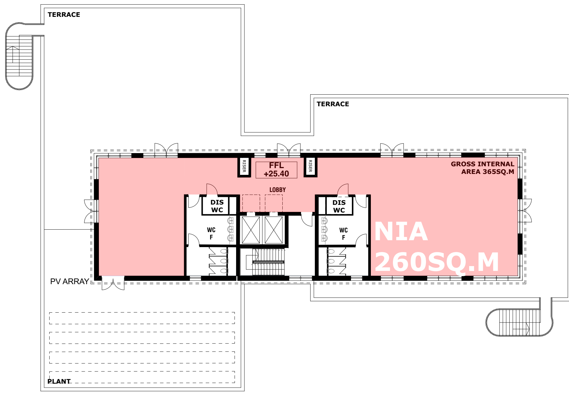
THIRD FLOOR
