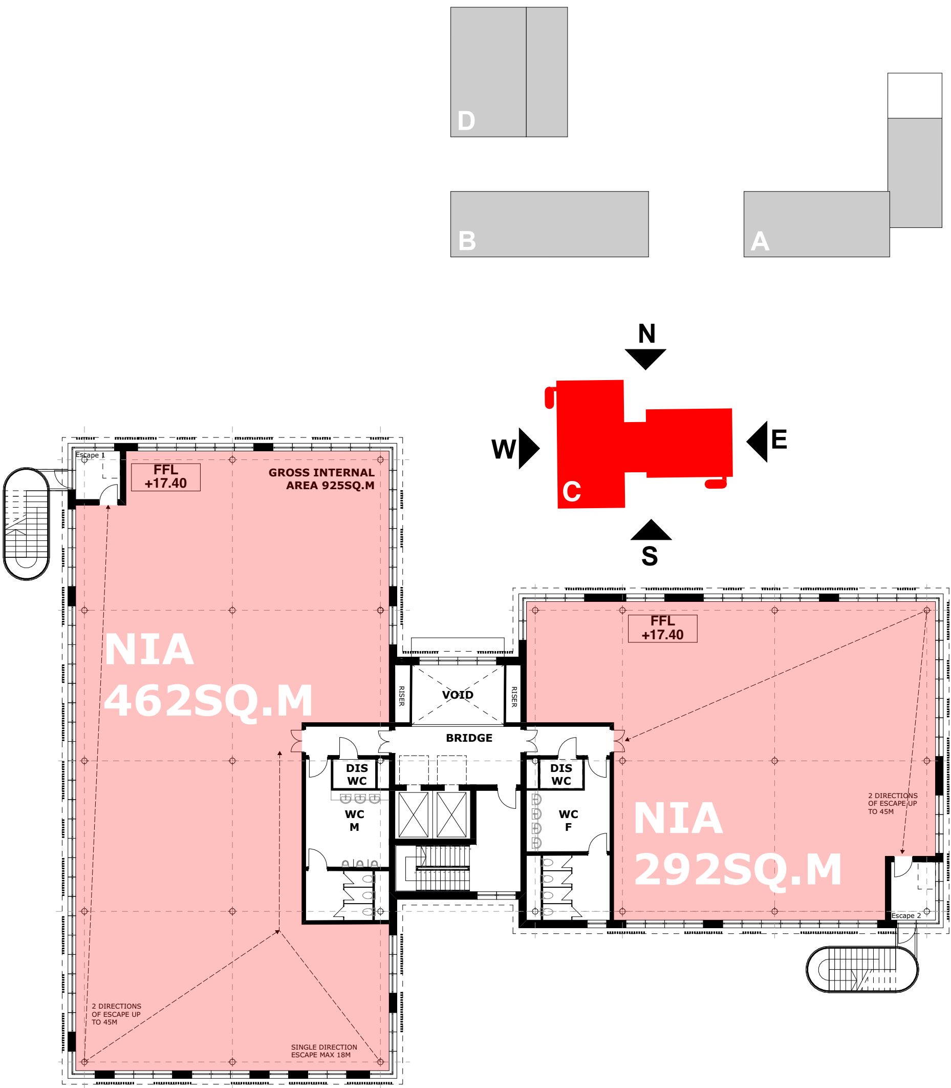
FIRST & SECOND FLOOR
