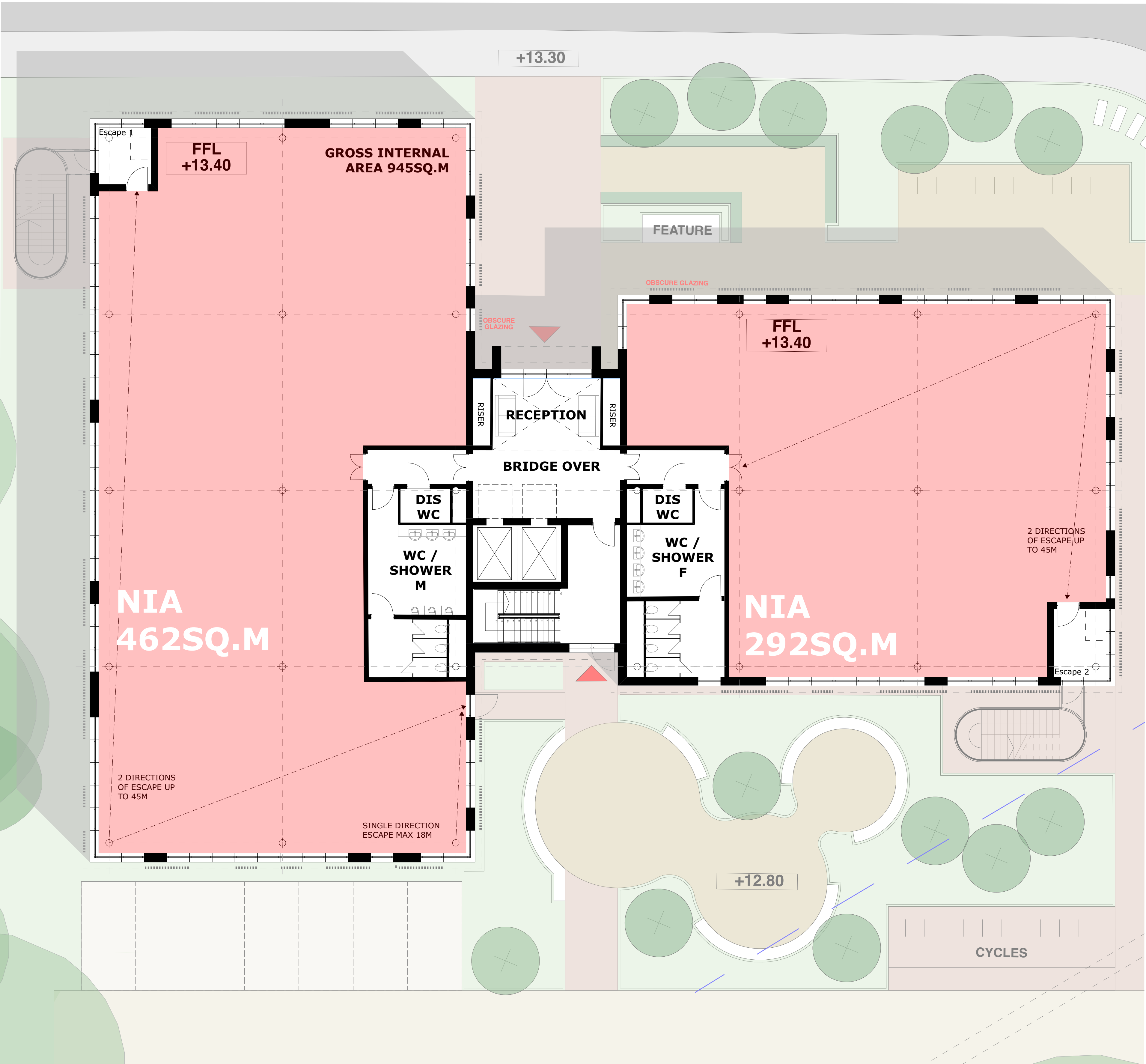
GROUND FLOOR
