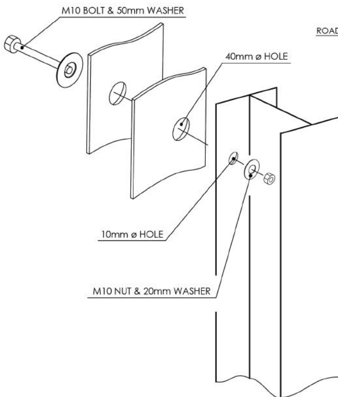
FASTENING SHEETS
