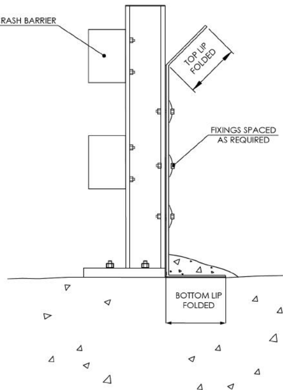
SECTION VIEW
