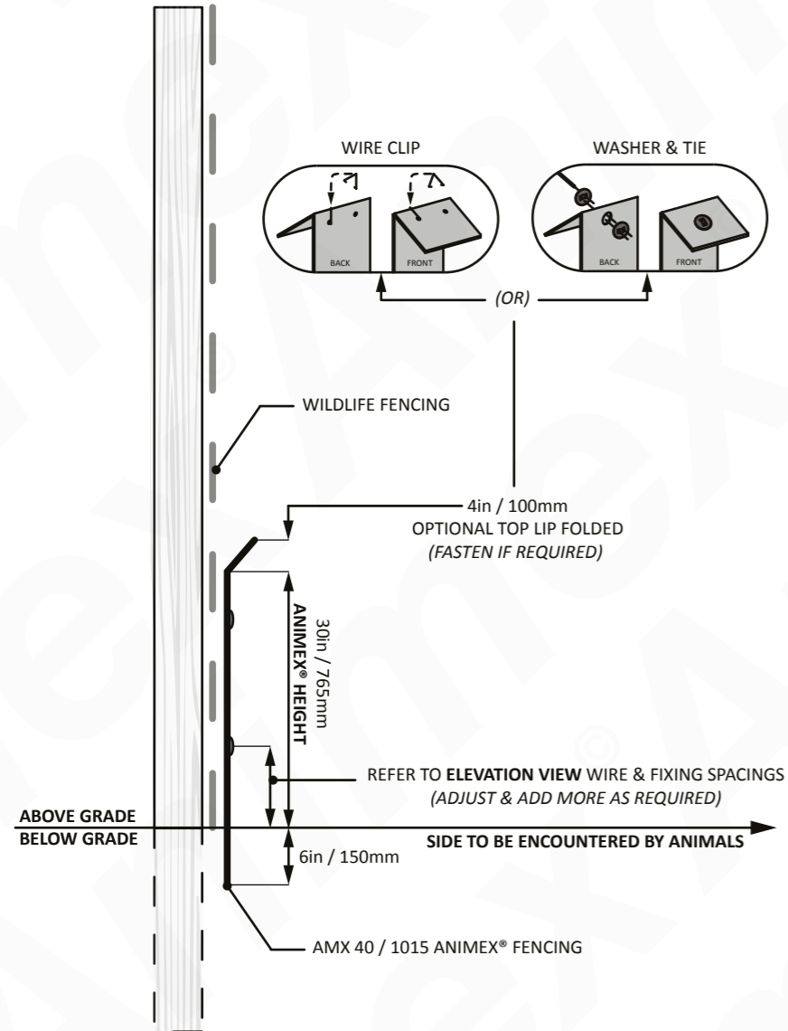
SECTION VIEW SCALE 1:20
