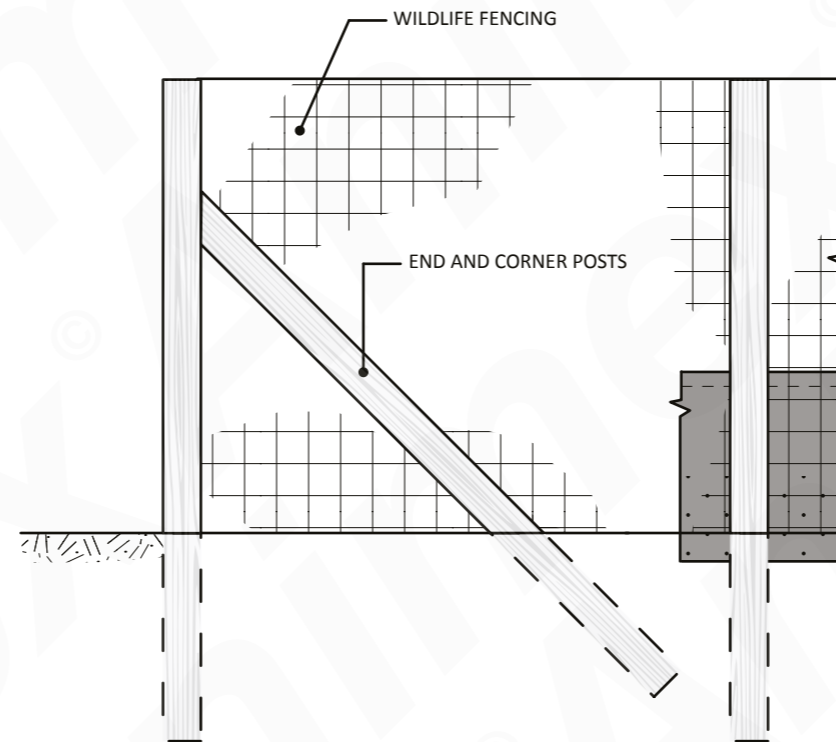
ELEVATION VIEW SCALE 1:40
