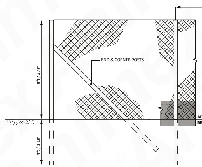
ELEVATION VIEW SCALE 1:40
