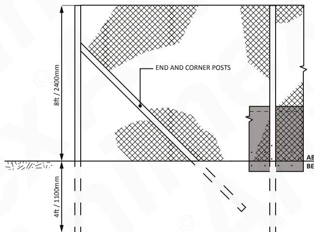
ELEVATION VIEW SCALE 1:40
