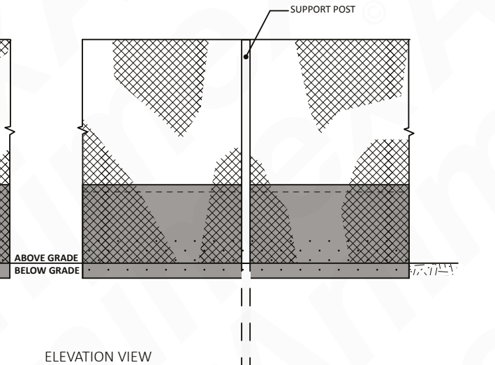
ELEVATION VIEW SCALE 1:40
