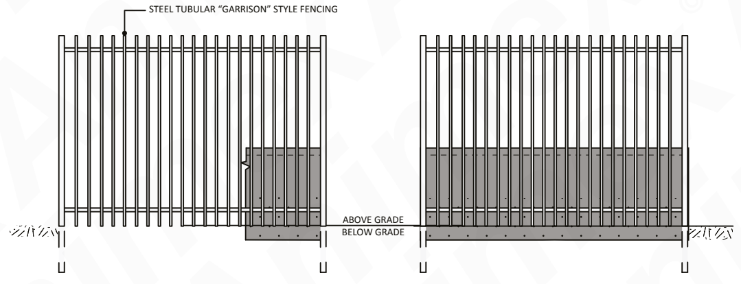
ELEVATION VIEW SCALE 1:40
