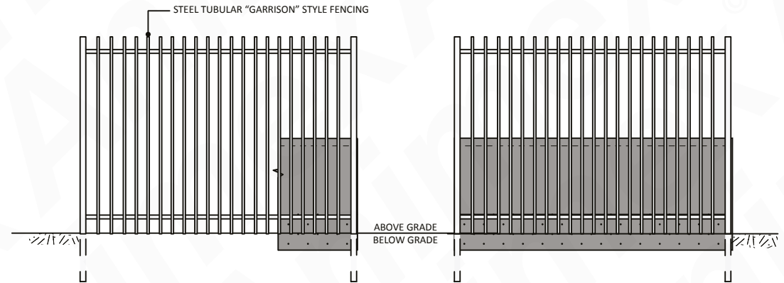
ELEVATION VIEW SCALE 1:40
