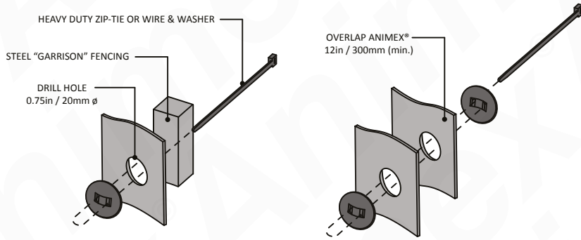
ATTACHING & JOINING SECTIONS SCALE 1:4
