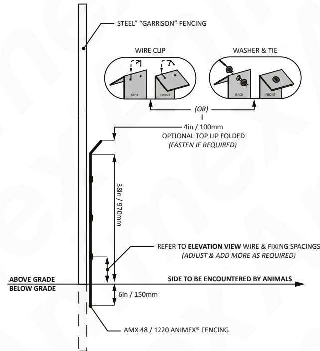
SECTION VIEW SCALE 1:20
