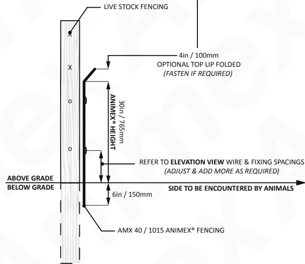
SECTION VIEW SCALE 1:20
