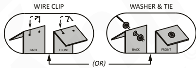
ATTACHING & JOINING SECTIONS SCALE 1:4
