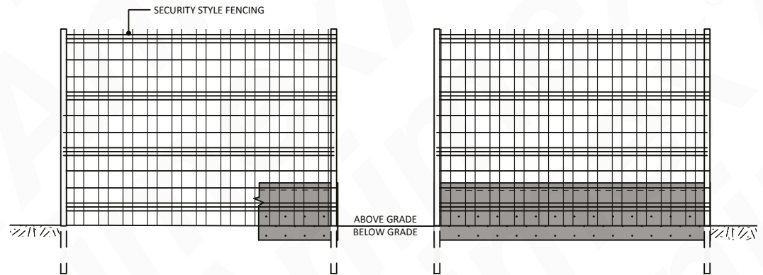
ELEVATION VIEW SCALE 1:40
