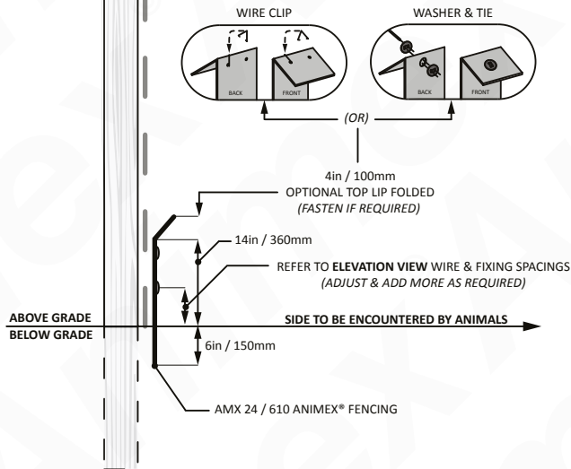
SECTION VIEW SCALE 1:20
