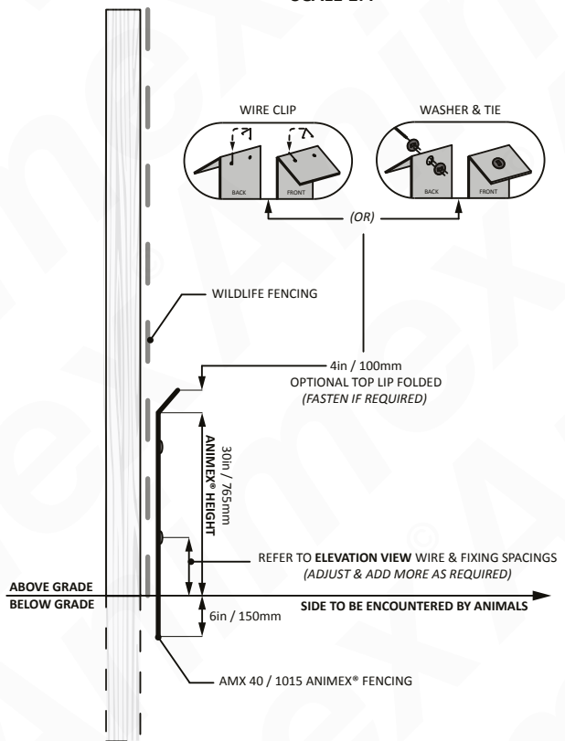
SECTION VIEW SCALE 1:20
