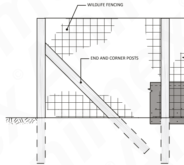
ELEVATION VIEW SCALE 1:40
