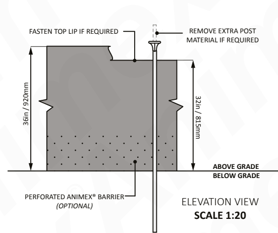
ELEVATION VIEW SCALE 1:20
