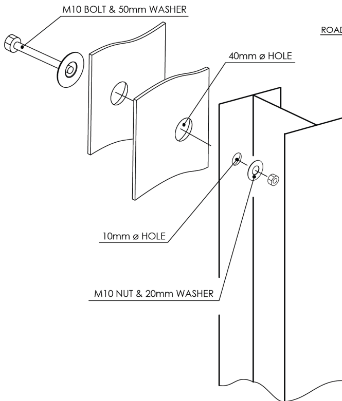
FASTENING SHEETS DO NOT OVER TIGHTEN
