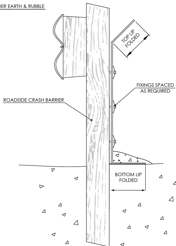
SECTION VIEW
