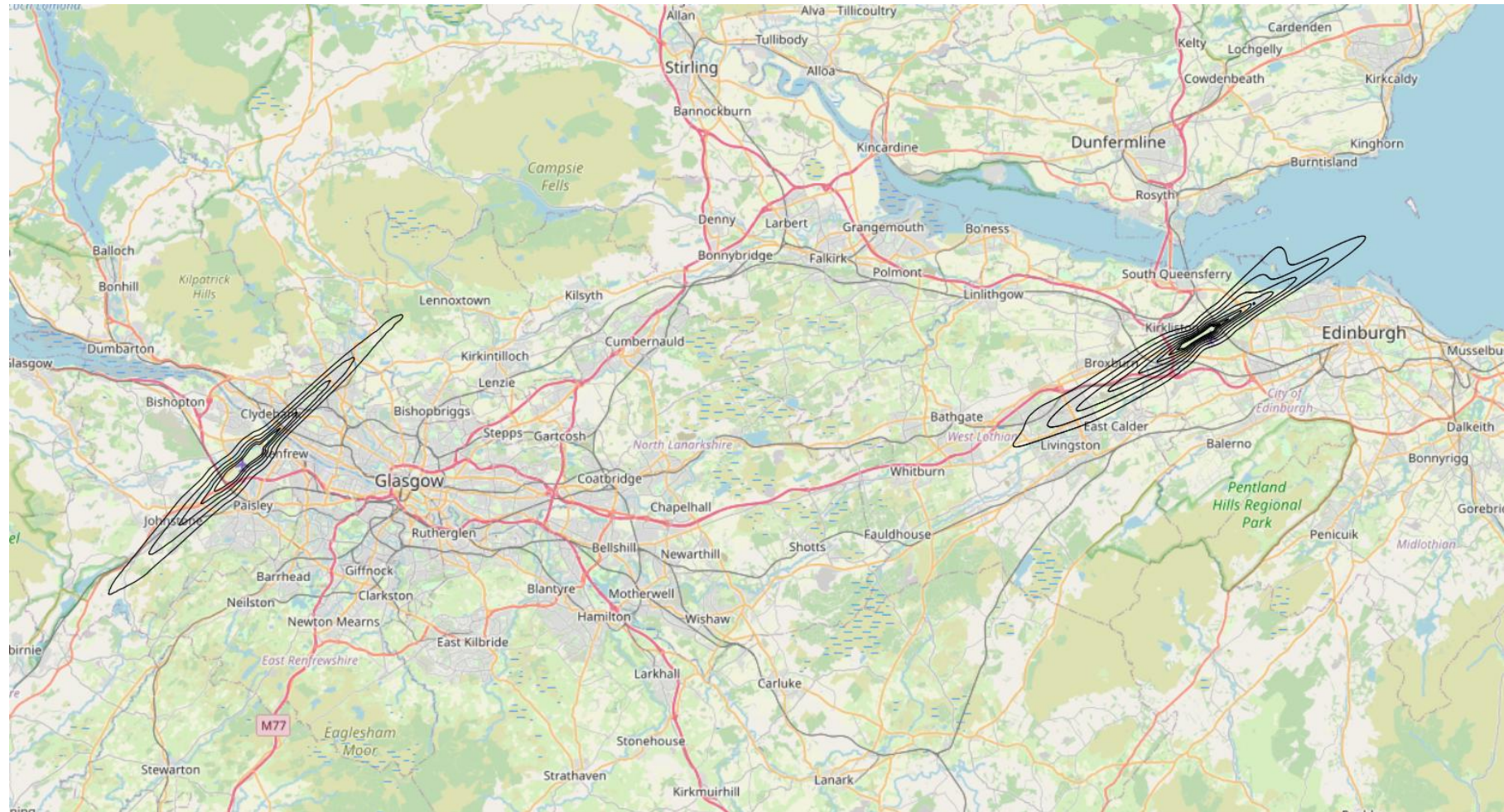
Figure 21: L_{Aeq, 16 Hr} Daytime Cluster Wide “Without Airspace Change” Baseline, 2027
