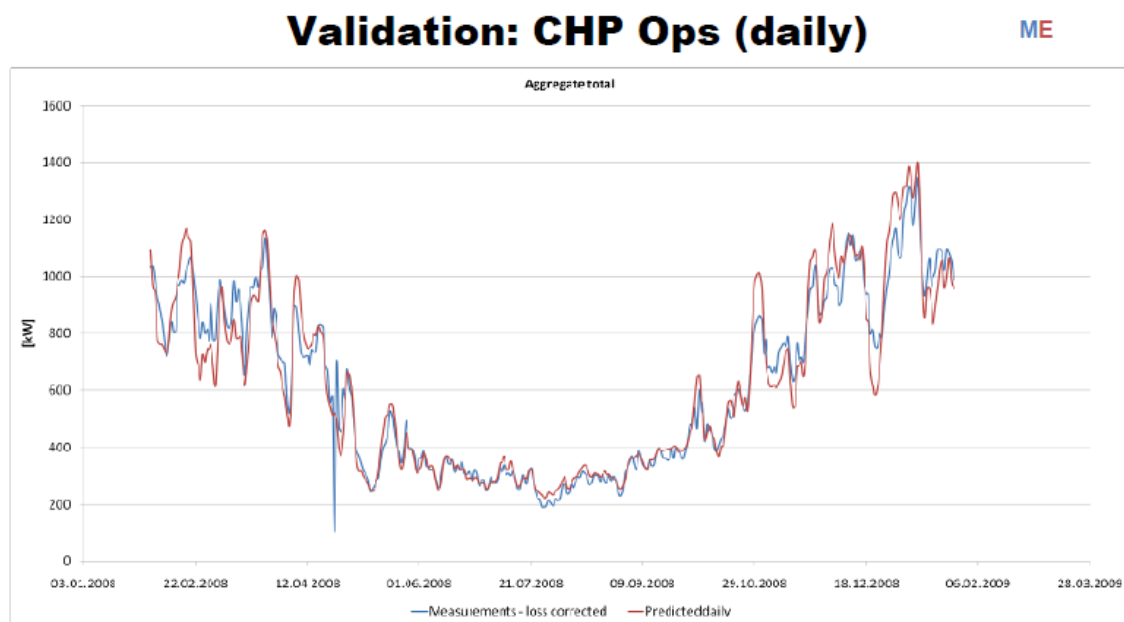
Figure 3.2 – Comparison of predicted and actual heat demands for a site in London
