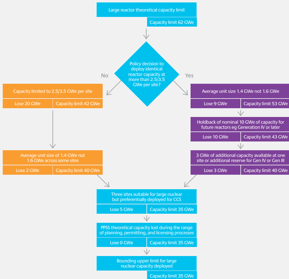
FIGURE 7 Flow chart showing the reduction from theoretical large reactor capacity to an upper bounding limit for generation III+ large reactor capacity deployed by 2050
