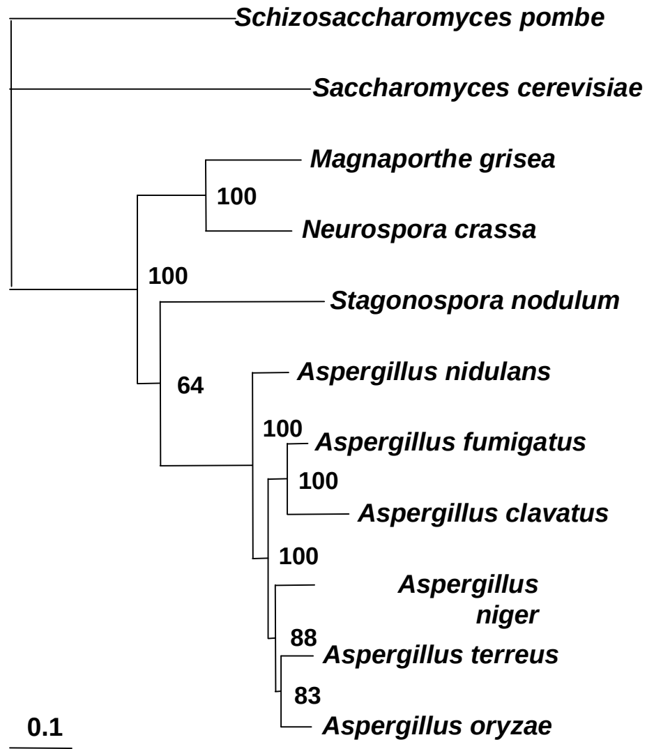
Supplementary Figure 1 Phylogeny of filamentous fungi. Maximum likelihood tree based on concatenation of twenty orthologous proteins (Supplementary Table 3). Branch length and likelihood values were calculated by TREE –PUZZLE and indicate substitutions per site. Numbers at nodes are bootstrap values.
