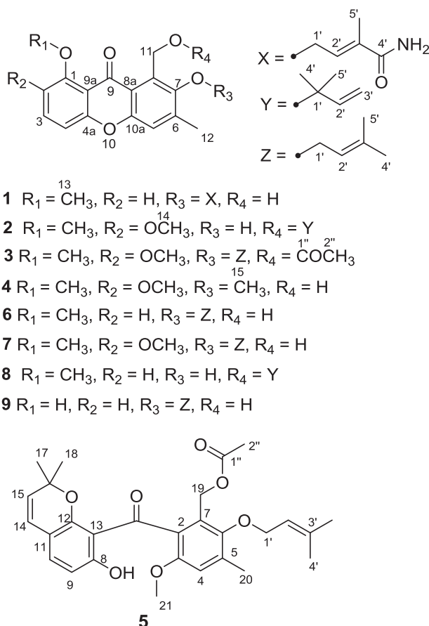
Figure 1 Chemical structures of compounds 1–9.
