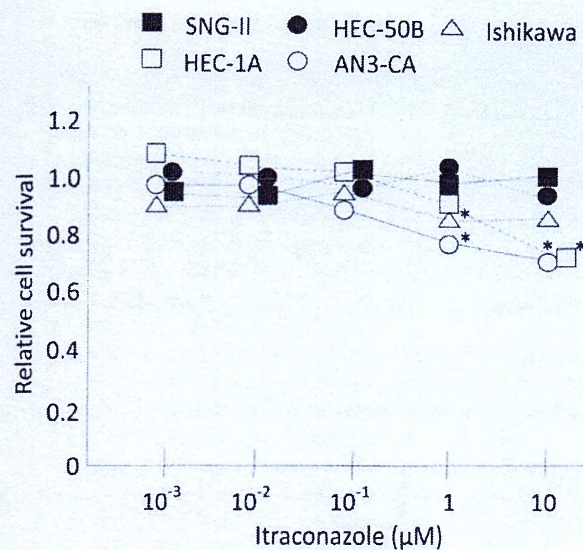
Figure 1. Proliferation of EC cells. Five EC cell lines were cultured with indicated concentrations of itraconazole for 48 h, and cell viability was evaluated with the MTT assay. Results were compared to those of the vehicle-treated control group with the Mann-Whitney U-test. * p < 0.05 .
