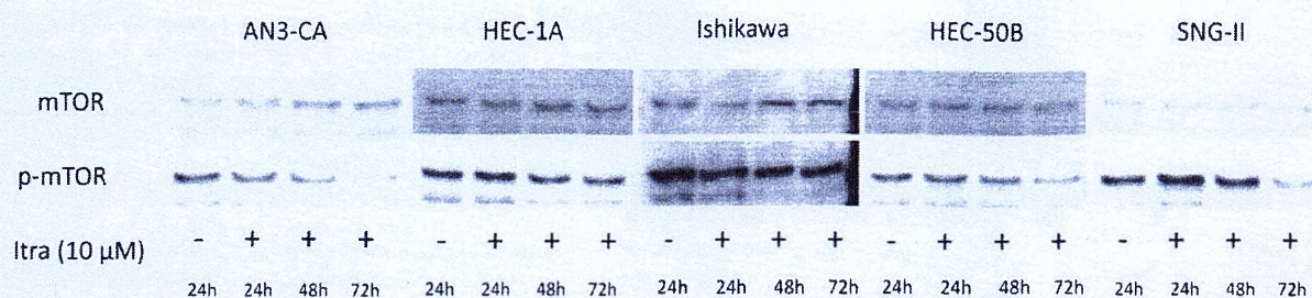
Figure 2. Itraconazole suppresses mTOR signaling. Cells were cultured with 10 \mu M itraconazole (Itra) for 24, 48, and 72 h and with vehicle for 24 h; protein expression was then analyzed by western blotting.
