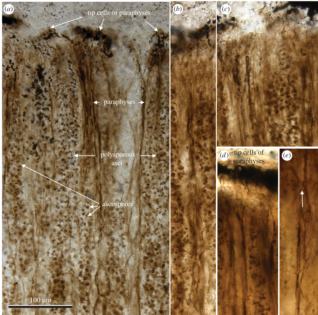
Figure 4. (a–e) Prototaxites aff. taiti from Rhynie chert, details from the longitudinal section in slide no. 149 CT B (figure 3). Polysporous asci and thin-walled, delicate paraphyses. The darkly pigmented epihymenial layer is best visible in (d). The arrow in (e) points to anastomosing paraphyses. Same magnification in (a–e).
