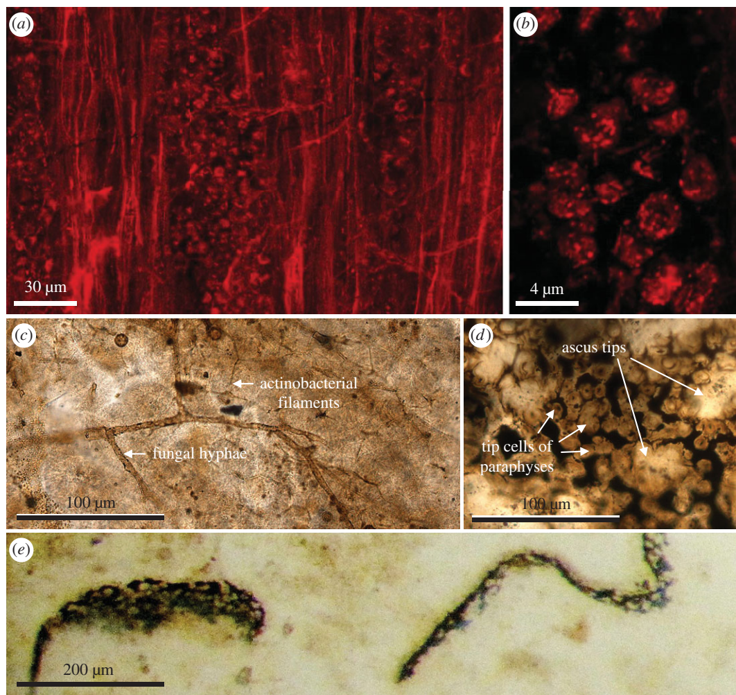
Figure 5. Prototaxites aff. taiti from Rhynie chert, details from slide no. 149 CT B; (a,b) confocal laser microscopy, (c–e) bright field light microscopy. (a) Detail of the hymenial layer with asci, paraphyses and invasive, contaminating fungal filaments. (b) Spores inside an ascus. (c) Contaminating fungal and bacterial filaments growing below the hymenial layer. (d) Laminar view, and (e) tangential (left) and cross-section (right) of detached fragments of the epihymenial layer, with tip cells of paraphyses and open ascus tips, the interspace being filled with dark pigments.
