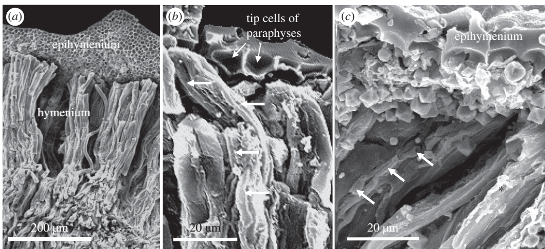
Figure 7. SEM micrographs of the charcoalified fragment of the hymenial layer of Prototaxites sp. (HD(L)171/03) from Welsh Borderland, lateral view. ( a ) The dense epihymenial layer is partly peeling off (figure 5 a, b ). ( b ) Detail of the hymenial layer with immature asci. Arrows point to presumed paraphyses and/or fungal or bacterial invaders. ( c ) Arrows point to remains of a few thin-walled paraphyses. The asterisk points to an ascus with superficial impressions of lost paraphyses.
