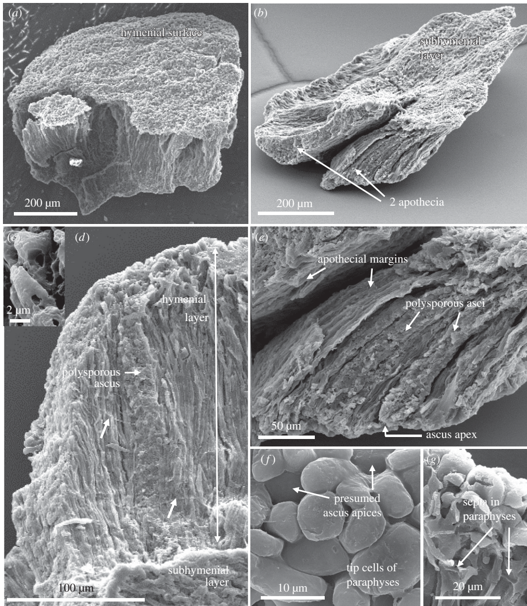
Figure 8. SEM micrographs of a charcoalified apothecial fragment from the Late Silurian (LL03/02) from Ludford Lane, Shropshire. (a) Upside-up, and (b, e) upside-down positional views of the specimen. (c) Presumed crozier in the basal part of the hymenial layer. (d) The longitudinally fractured hymenial layer is built up by slim, unbranched paraphyses. The numerous ascospores within the fractured, polysporous ascus reveal irregular outlines, i.e. are deformed. Arrows point to bacterial contaminants which had grown post-mortem over the fragment. (e) Detail of surface in (b): the thin apothecial margin is built up by parallel hyphae. (f) The rounded tip cells of paraphyses are grouped around presumed ascus apices. (g) Septa are visible in fractured paraphyses.
