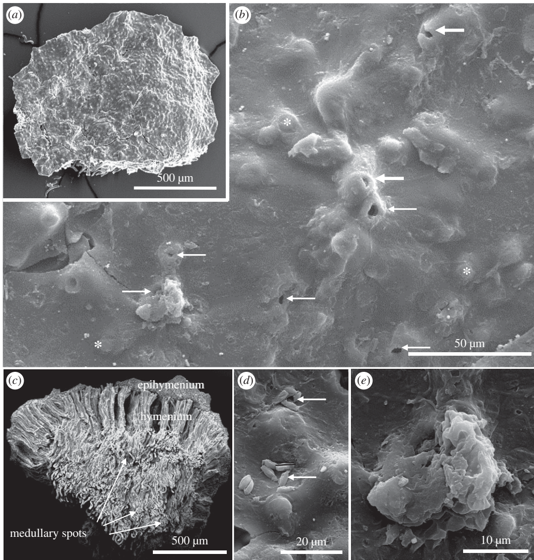
Figure 6. SEM micrographs of a charcoalified fragment of the hymenial layer of Prototaxites sp. (HD(L)171/03) from Welsh Borderland. ( a, b, d, e ) Laminal view of the surface. ( a ) Overview; ( b ) detail of the hymenial surface. The asterisks mark an ascus apex prior to dehiscence. Thick arrows point to asci shortly after ascospore release, the inoperculate ascus tips having slightly expanded and opened with a slit. Thin arrows point to empty asci whose wall sank back into the hymenial layer. ( c ) Lower surface of the specimen. ( d ) Arrows point to shrivelled, presumed ascospores after landing on the hymenial surface. ( e ) Presumed ascospores having germinated next to the apex of the empty ascus.
