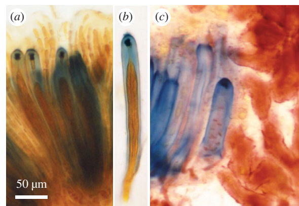
Figure 10. Light micrographs of iodine-stained free-hand sections of the ascoma (apothecium) of extant Peltigera spp. (lichenized ascomycetes) whose ascus wall differs structurally and chemically from ascospores, paraphyses and vegetative hyphae. (a) Detail of the hymenial layer of P. canina and (b) mature ascus with eight spindle-shaped, three-septate ascospores, both stained with Lugol's solution (IKI). (c) Detail of the hymenial layer and adjacent margin of P. venosa subjected to the van Wisselingh test for chitin (red coloration of chitosan after hydrolytic transformation of chitin). Red coloration, indicative of chitin, is discernible in the walls of vegetative hyphae of the apothecial margin, of paraphyses and of the ascospores. In both preparations, the ascus wall stains blue with iodine due to amyloid compounds (presumably lichenin-like glucans with \beta -1,3 and \beta -1,4 linkage bonds).
