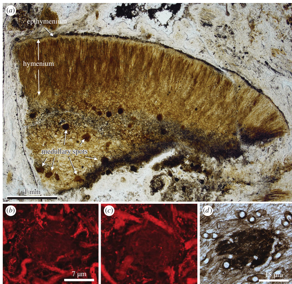
Figure 1. Petrographic thin section of Prototaxites taiti in bright field ( a ) and confocal laser microscopy ( b,c ), and peel in bright field microscopy ( d ). ( a–c ) The type specimen of P. taiti from the Rhynie cherts, new photograph of slide no. 2525 of the Kidston Collection. ( a ) This fragment is depicted in black and white in Kidston & Lang [3] in fig. 113, with the following legend: 'View of one of the sections of the second fragment which shows the peripheral tissues'. Here these peripheral tissues are interpreted as the hymenial layer of the ascoma of an ascomycete, the section plane being slightly tangential. Note the innumerable silicate crystals, best visible outside the tissues. ( b–d ) Medullary spots: in confocal laser microscopy ( b,c ), (slide no. 2525), intense wefts of hyphae in close contact with a population of minute cells visible in bright field microscopy ( d ), (slide 149 B 3).
