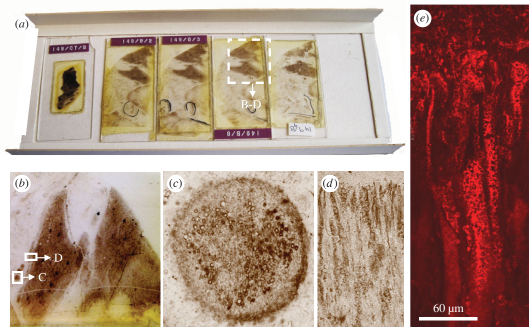
Figure 2. Slides of a petrographic thin section and a series of peels of Prototaxites taiti , from Rhynie chert as prepared by Prof. AG Lyon. (a) Overview of petrographic thin section 149 CT B (see details in figures 3–5) and serial peels in slides 149/B 2, 3, 8 & 9. (b) Detail of slide 149/B 8, the position of figures (c) and (d) being marked. (c) Cross-section of a cord (or a very young axis?) with a somewhat denser peripheral zone. (d) Slightly tangential section of the peripheral layer of a ‘fleshy’ axis which, in the present study, is interpreted as the hymenial layer of an apothecium-bearing ascomycete. (e) Confocal laser micrograph of the hymenial layer of the type specimen of P. taiti (slide no. 2525 of the Kidston and Lang collection; see figure 1a), showing the tubes, i.e. asci with ascospores, in the hymenial layer.
