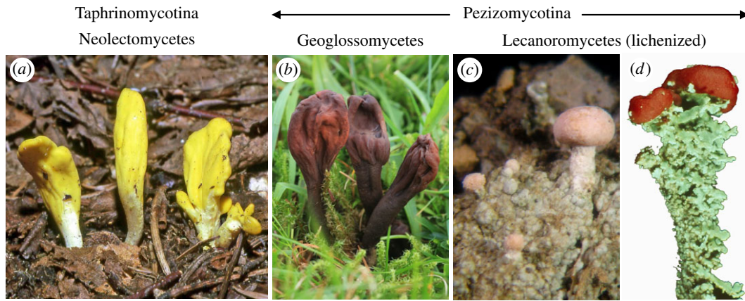
Figure 9. Extant ascomycetes with clavate to roundish sporophores (ascomata). (a) The presumably saprotrophic Neolecta vitellina , one out of four species of Neolectomycetes, the only Taphrinomycotina with ascomata. The extensive hymenial layer is bright yellow. Photo courtesy of Raymond McNeil. (b) The saprotrophic dark-purple earth tongue ( Geoglossum atropurpureum , syn. Thuemenidium a. ). Photo courtesy of Knud Knudsen. (c) The stalked, non-lichenized ascomata of Dibaia baeomyces (syn. Baeomyces roseus ) growing out of the crustose lichen thallus. (d) Convex ascomata of Cladonia bellidiflora with red coloration (due to crystals of the anthraquinone bellidiflorin in the epihymenial layer) on an erect podetium whose surface is covered by dorsiventrally organized, lichenized squamules.
