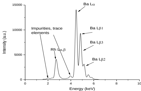
Figure 24. EDXRF spectrum of barium hydroxide.
