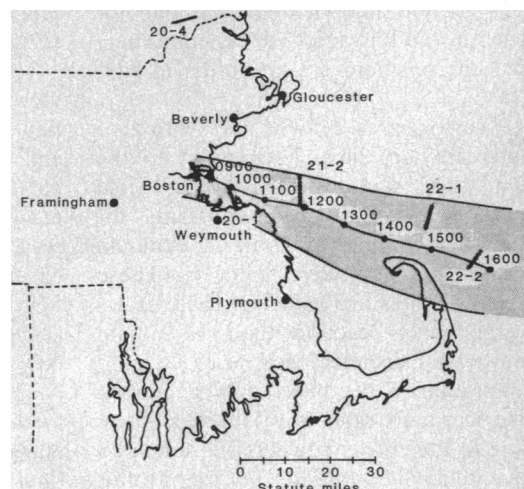
Fig. 1. Air parcel trajectory and aircraft sample positions for 18 August 1978 (at right). The plot at left shows the \text{O}_3 profile and integrated sample collection interval for the most distant plume traverse; ppb, parts per billion.
