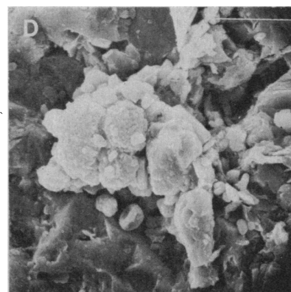
Fig. 2. (A–D) Scanning electron micrographs of the microcolonial structures from rocks shown in Fig. 1. The appearance of structures in (A) differs from those of the others. The subunits on (B), (C), and (D) are about 5 \mu\text{m} in diameter. Scale bar for (A), (B), and (C), 50 \mu\text{m} , and for (D), 10 \mu\text{m} . (E) Thin section of a microcolonial structure from a granite specimen from the Sonoran Desert. Mitochondria and nuclear membranes can be observed. The dark circular structures appear to be concentric bodies (8). Dense granular material is present in the areas between cells and especially on the external region of the cells. Scale bar, 1.0 \mu\text{m} .
