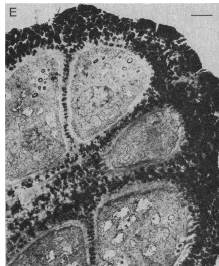
Fig. 2. (A–D) Scanning electron micrographs of the microcolonial structures from rocks shown in Fig. 1. The appearance of structures in (A) differs from those of the others. The subunits on (B), (C), and (D) are about 5 \mu\text{m} in diameter. Scale bar for (A), (B), and (C), 50 \mu\text{m} , and for (D), 10 \mu\text{m} . (E) Thin section of a microcolonial structure from a granite specimen from the Sonoran Desert. Mitochondria and nuclear membranes can be observed. The dark circular structures appear to be concentric bodies (8). Dense granular material is present in the areas between cells and especially on the external region of the cells. Scale bar, 1.0 \mu\text{m} .
