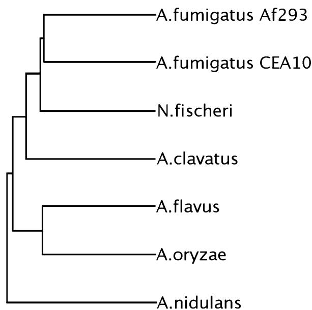
Fig. 1 Phylogenetic tree of five Aspergillus spp. A set of 1000 ortholog clusters containing a single representative from each of the genomes analyzed with consistent protein lengths was used to generate a phylogenetic tree. The blastP bit scores were converted to a distance metric, and the Phylip package was used to create the tree using the UPGMA method.
