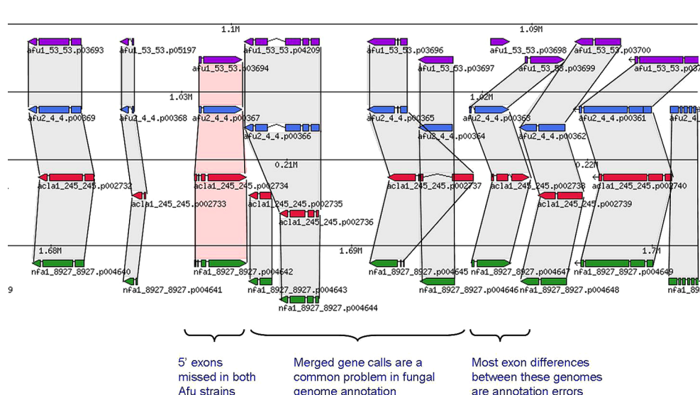
Fig. 3 Detailed synteny view highlighting annotation errors. This zoomed-in view of a syntenic block, in which individual gene structures are visible, shows some of the data inconsistencies that can adversely affect automated comparative analyses. Aspergillus fumigatus Af293 genes are colored purple, A. fumigatus CEA10 genes are colored blue, Neosartorya fischeri genes are colored green and A. clavatus genes are colored red.
