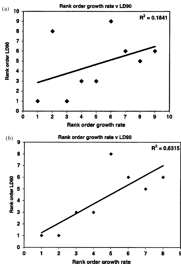
Fig. 2 Rank order of LD 90 versus rank order of growth rate for Aspergillus fumigatus isolates (a) including Af65 (second fastest grower in vitro , x-axis) and (b) excluding Af65. Regression analysis was performed on both plots, demonstrating an improved correlation between the parameters following the removal of Af65.
