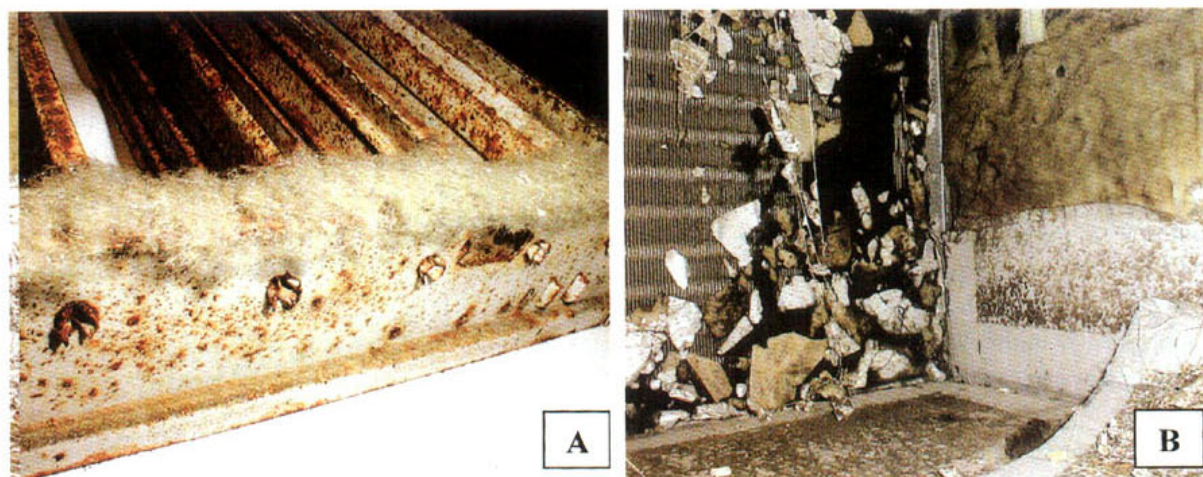
Figure 4. A, Operating room diffuser showing fiberglass fragments from insulation blown downstream from a variable airflow volume (VAV) unit. Severe rusting is indicative of intermittent or chronic condensation. B, Interior view of a VAV unit showing deterioration of foil-lined fiberglass insulating material.
