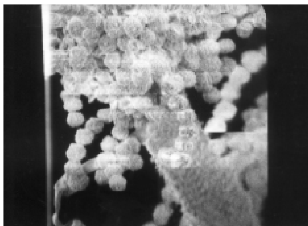
Figure 1. Scanning electron micrograph of a toxigenic strain of A. flavus showing rough conidia and conidiophore wall, \times 910 .
