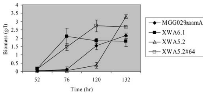
Fig. 2 Growth curve of various A. niger strains in batch culture using 1% (w/v) starch as sole carbon source. Biomass production of MGG029- \Delta aamA, XWA6.1, XWA5.2, and XWA5.2#64 was determined at several time points during growth (52, 76, 120 and 132 h after inoculation of equal amounts of spores). Dry cell weight measurements were performed in duplicate from two independent cultivations. The error bars indicate the standard deviation of the mean dry weights
