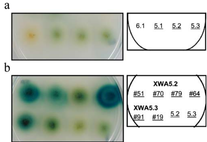
Fig. 3 Plate assay for analysis of laccase (Pox2) production. a ABTS overlay assay on MGG029- \Delta aamA transformants, containing the GlaA2::Pox2 expression cassette (XWA5.1, 5.2, and 5.3) and the expression cassette with the catalytic part of glucoamylase only (XWA6.1). b Detection of laccase production using ABTS overlay assay for a selection of mutants that displayed a fast-growing phenotype on starch medium after UV mutagenesis. All colonies displayed in a and b are covered with ABTS overlay agarose and incubated at room temperature for 17 h. Strains showing the green color are positive for laccase activity. Strain positions are indicated in the drawn template and laccase-producing strains are underlined
